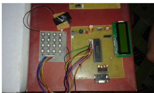
Fig.5 Receiver Unit
