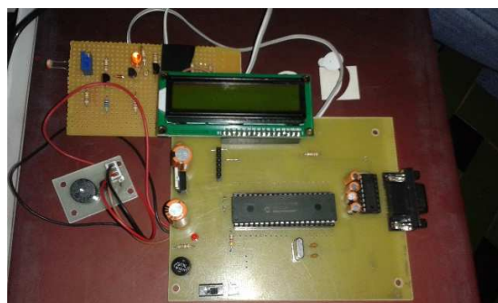
Fig 3 Transmitter Unit
