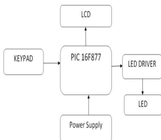
Fig.2 Block Diagram of Transmitter
