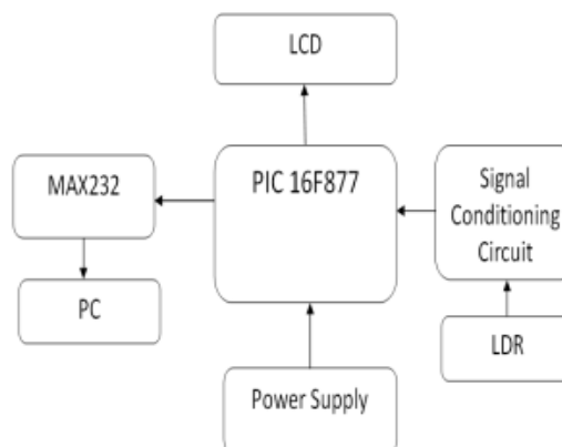
Fig.4 Receiver Section
